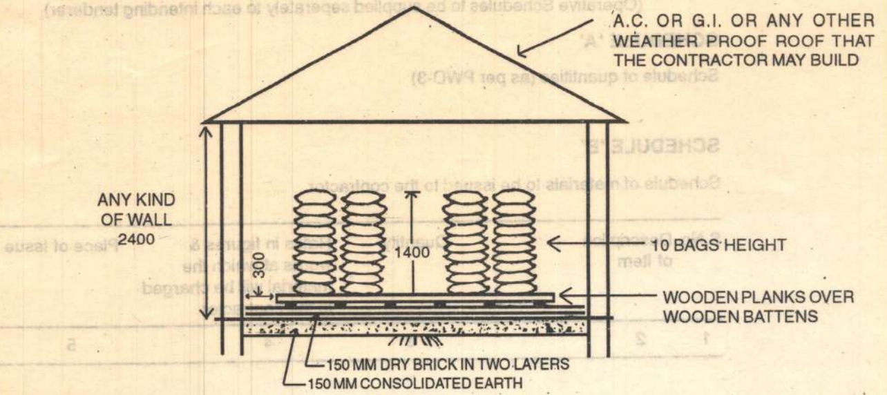
SECTION AB
